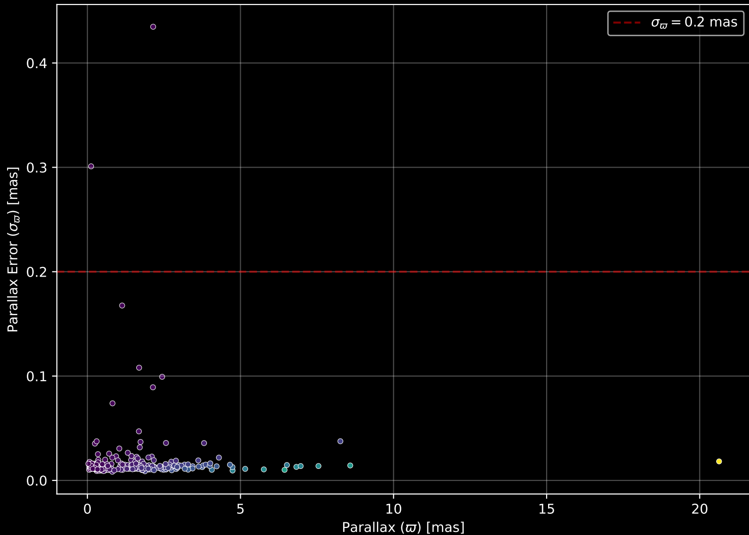
APOGEE DR17 Field: [240-12] Parallax Quality (n= 265)
