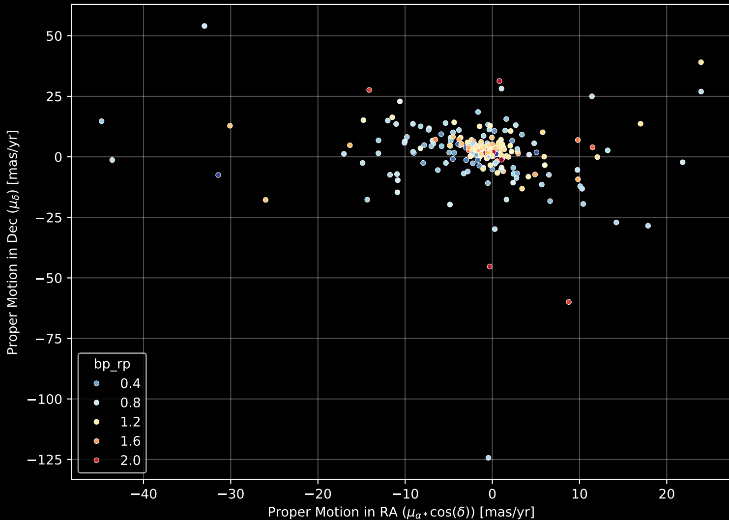
APOGEE DR17 Field: [240-12] Proper Motion Diagram (n= 265)
