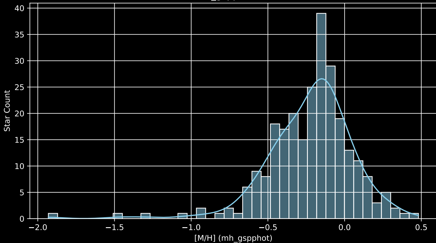
APOGEE DR17 Field: [240-12 [M/H] (mh_gspphot) (n= 259)
