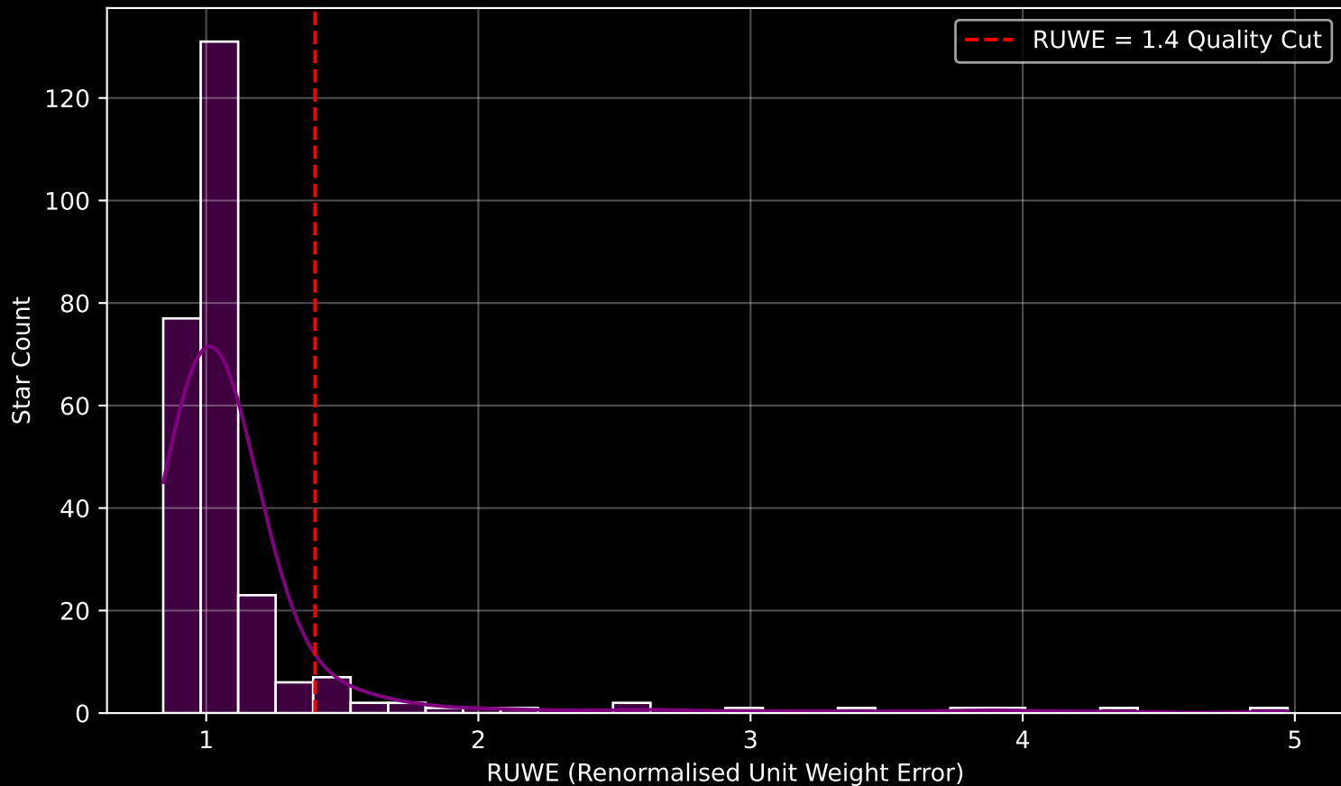
GAPOGEE DR17 Field [240-12] RUWE Distribution (n= 259)
